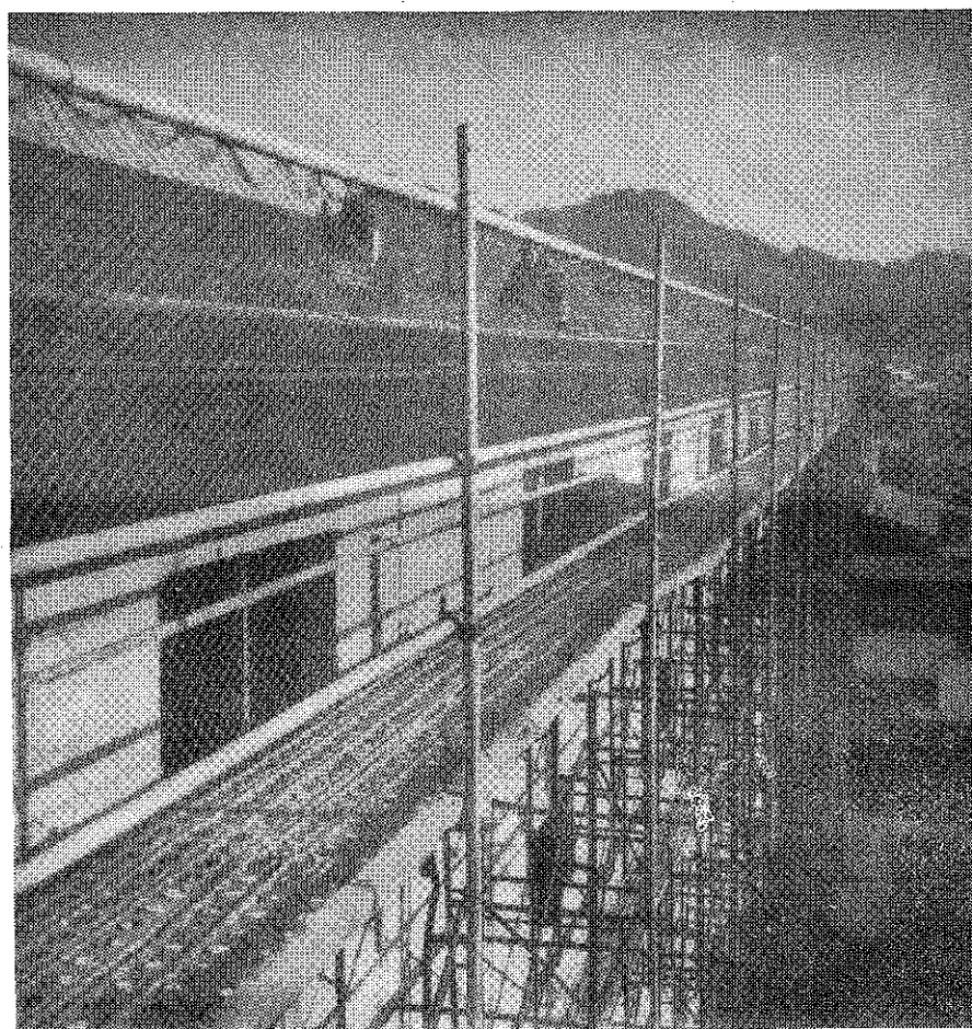
Scaffolding at 4 story UEPH under construction at Casey. Note that the guard rails exceed the level of the roof and is equipped with a catch net. A person working on the roof who accidentally slips will fall only 4 feet or less, also the net prevents loose material from falling the remaining four floors.
