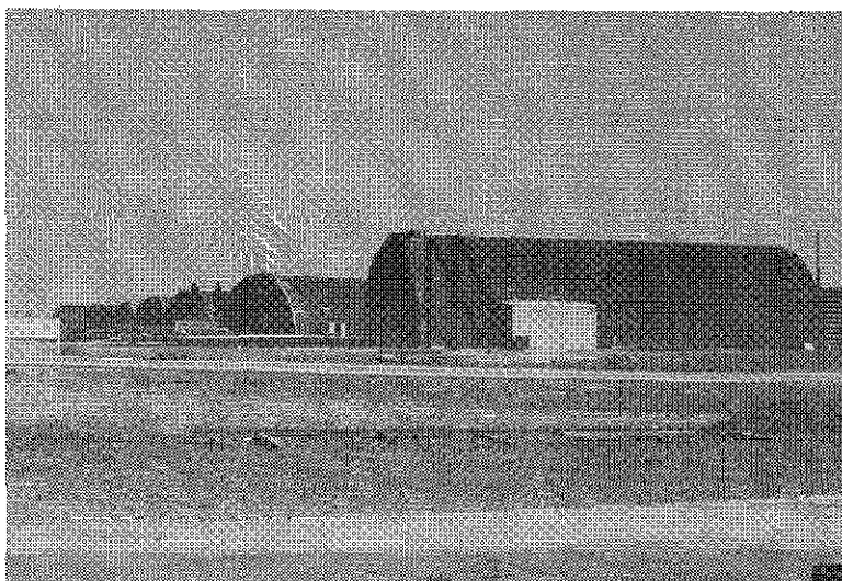
Aircraft shelter doors at Kunsan Air Base are about 85 percent complete. The contractor is Pum Yang Construction Co., Ltd.
