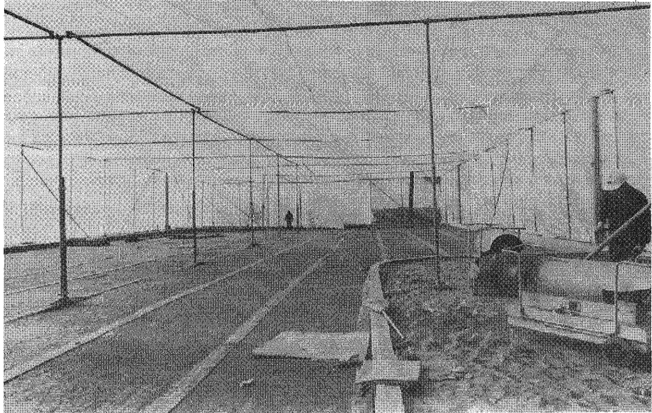
An elaborate cover and heaters are necessary for the winterization, which allow construction of the Yongsan Youth Activities Center parking lot to continue during the cold weather.
